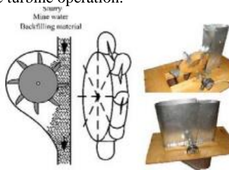
Fig. 1. The turbine for slurry (a), the wheel (b) and the pilot sample of the turbine for laboratory tests (c)
