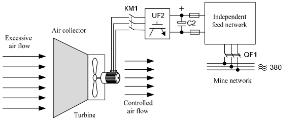
Fig. 3. The complete circuit diagram of air flow rate control with regeneration of current into the mine network
