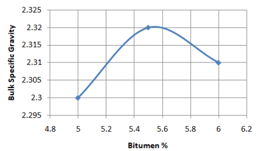
(c) BSG vs. Asphalt%
