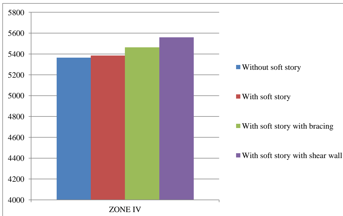
Fig Base shear in X direction for soft storey at bottom case for zone IV
