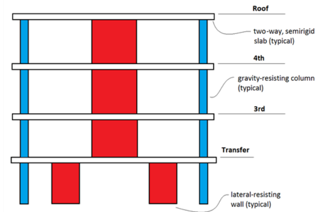
Fig. 1. Concept of the transfer systems in buildings.
