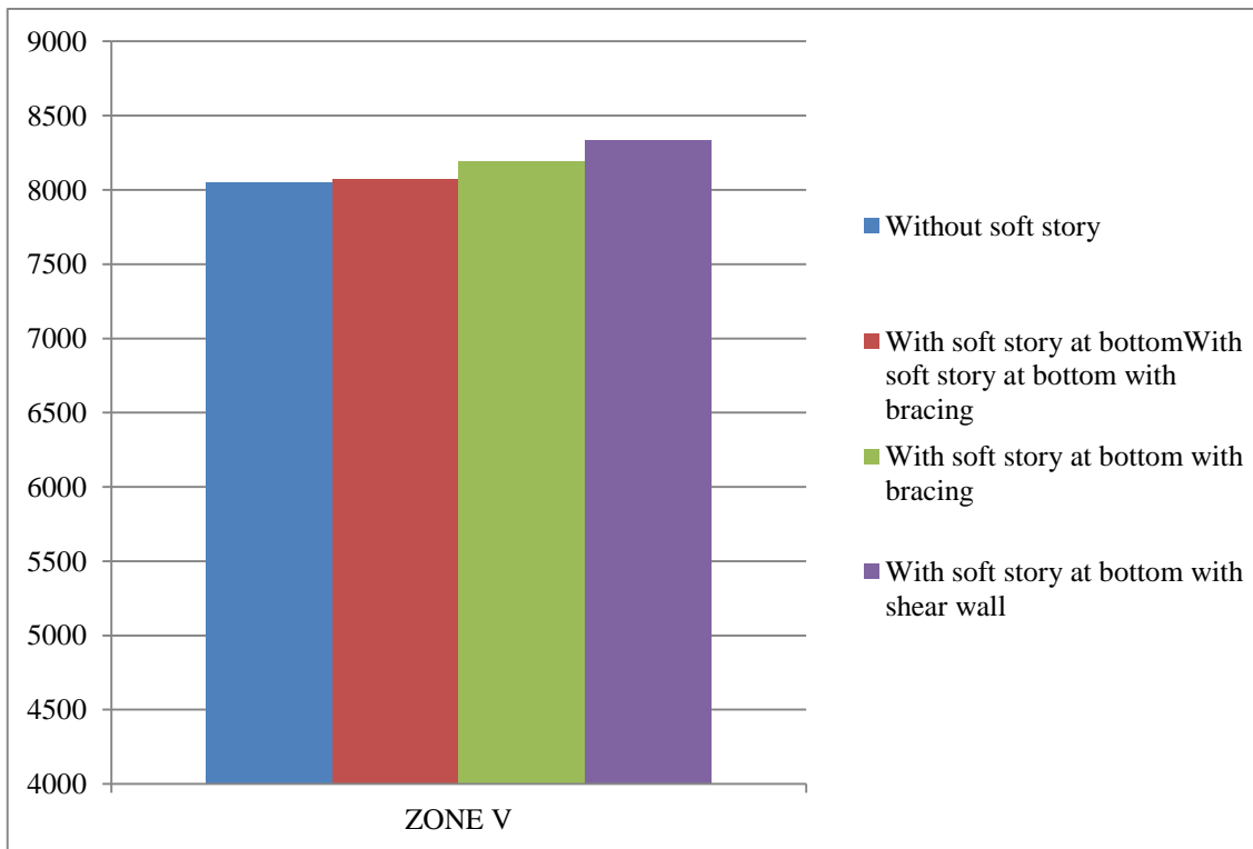
Fig Base shear in X direction for soft storey at bottom case for zone V
