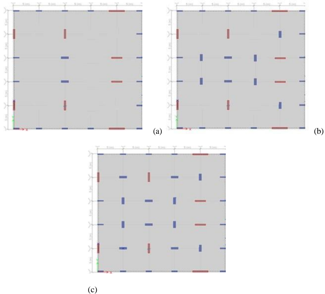
Fig. 2. Typical Plans with the locations of the planted columns (a) from ground to 1 st transfer level (b) between 1 st and 2 nd transfer levels (c) from 2 nd transfer level to roof.
