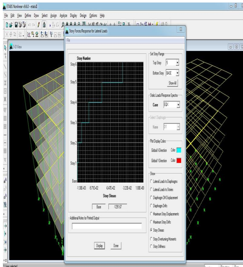
Fig. Base shear in ETABS for Zone II
