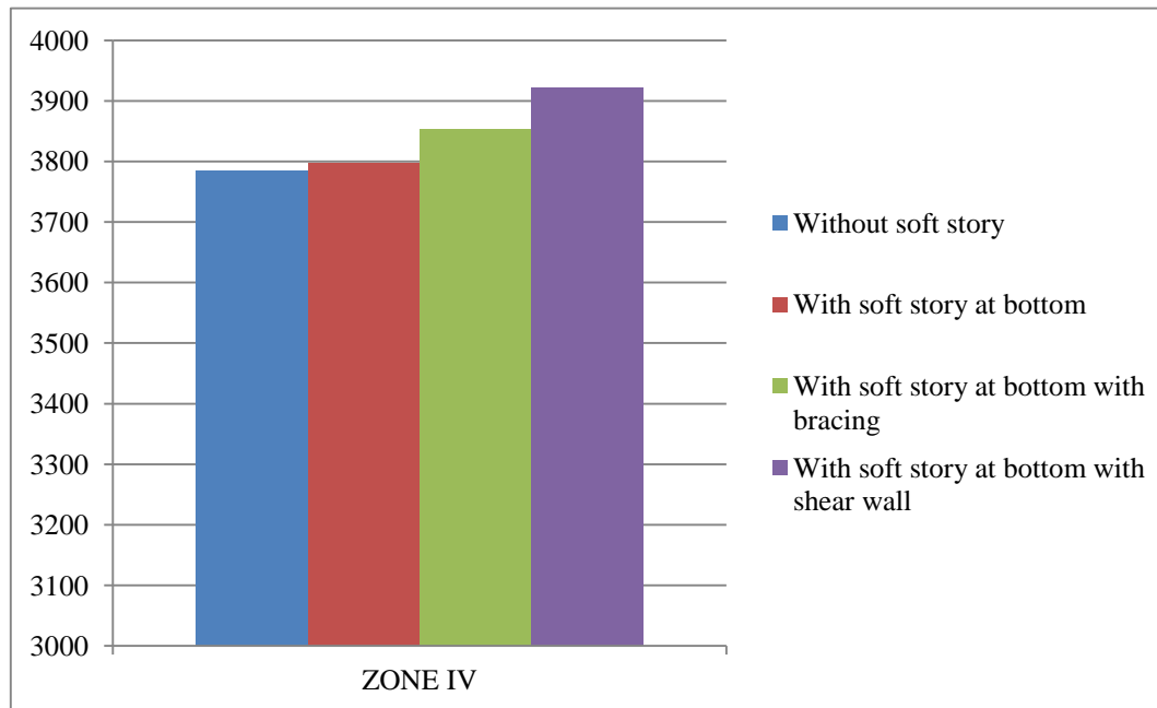
Fig. Base shear in Y direction for soft storey at bottom case for zone IV
