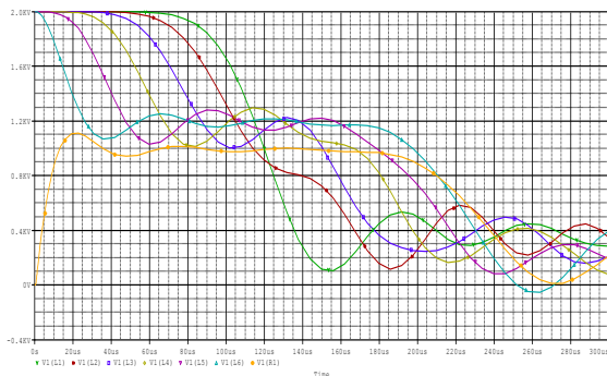
Fig. 9 The graph of the constituent capacitor bank voltages (2000V) and the resultant network voltage (1000V) that is available to the load (R1).
