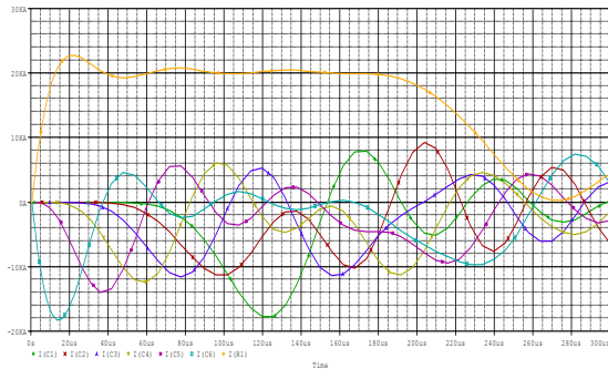
Fig.7 The output pulse current from Capacitor Bank C1, C2, C3, C4, C5, C6 and the resultant pulse current transferred to the load ( R1) at 258uS pulse duration. The resultant current pulse at the load is 20kA (20000A)
