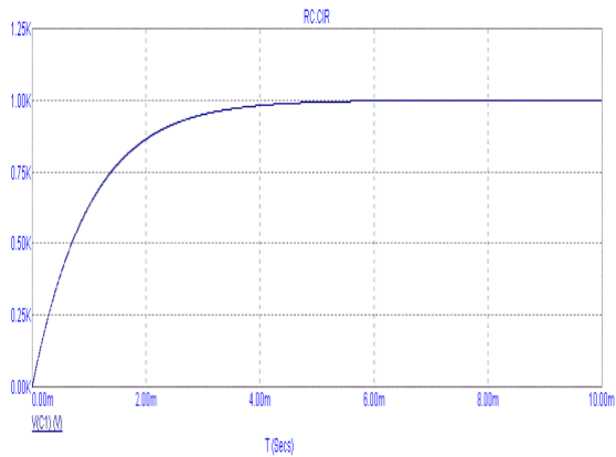
Fig. 2 Graph showing exponential voltage build-up in a charging capacitor (V (C1))
