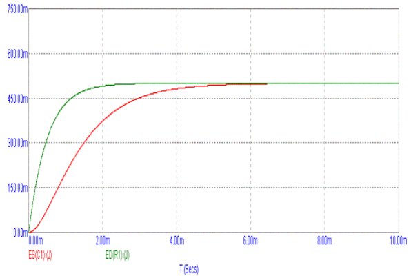
Fig. 4 Graph of energy stored and energy dissipated in a resistive charging circuit.
