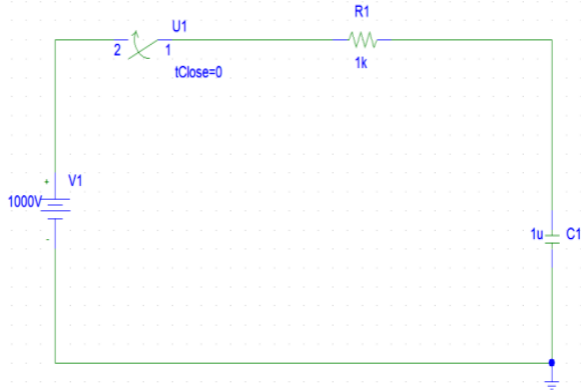
Fig. 1.RC Circuit model for charging a capacitor
