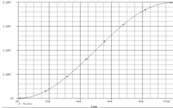
Fig. 5 Graph showing final network voltage of the inductive charging circuit
