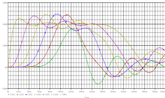
Fig. 8 The delayed output pulse current from inductors: L1, L2, L3, L4, L5, L6 and the resultant pulse current transferred to the load ( R1) at 258uS pulse duration. The resultant current pulse at the load is 20kA (20000A)
