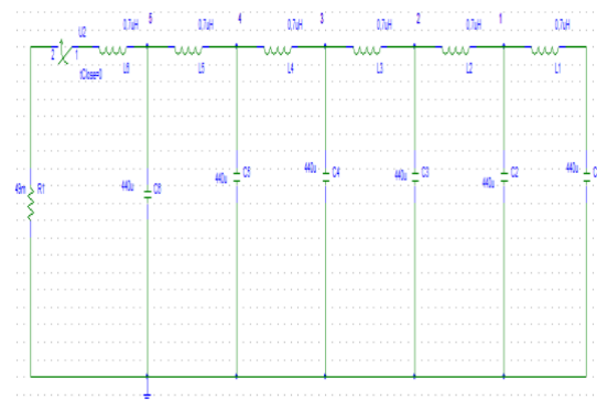
Fig. 6. Pulse Forming Network schematic at 49mΩ load impedance
